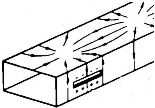
Slot excitation
