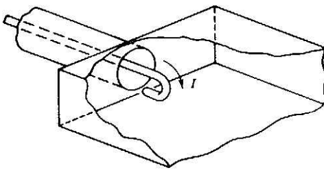
Loop excitation
