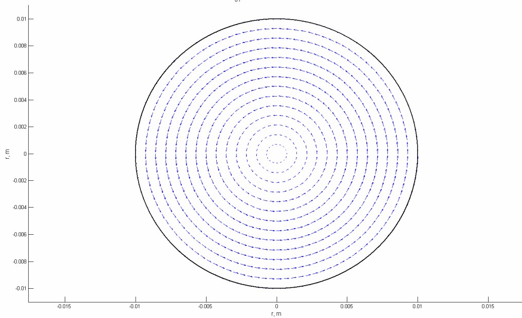
E_{01} , magnetinis laukas, z=\lambda/4
