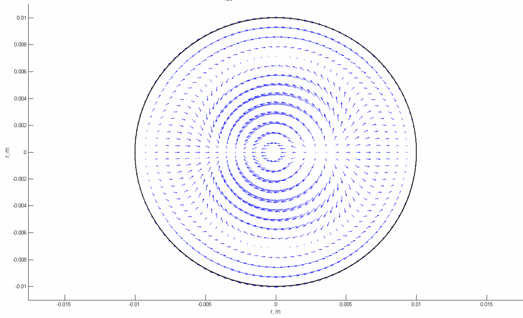
H_{123} magnetinis laukas, z=l/1 , t=T/4
