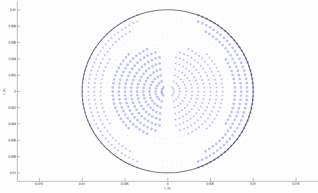
H_{123} magnetinis laukas, z=l/2 , t=T/4
